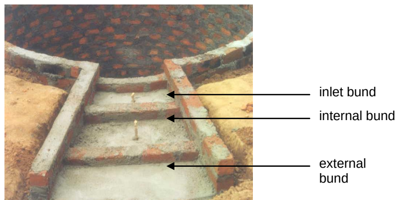
Figure 8: Bunds of the inlet before plastering
