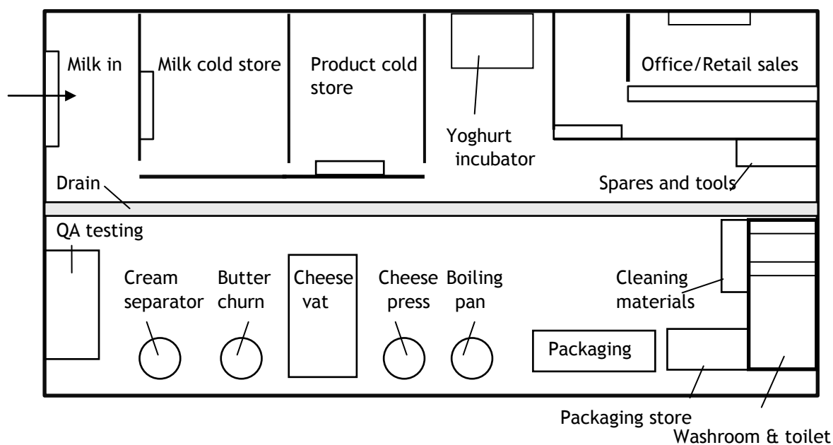
Figure 1: Layout of a small dairy
