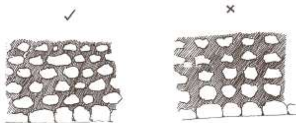
Figure 7: Break the joints, so you do not get lines of stones sitting on one another.
