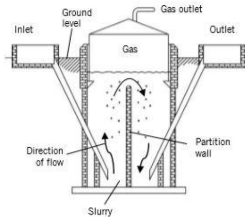
Figure 2: Floating cover digester Illustration: Practical Action / Neil Noble
