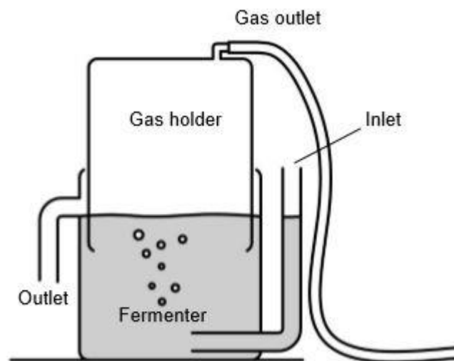
Figure 3: Compact biogas Illustration: Practical Action / Neil Noble
