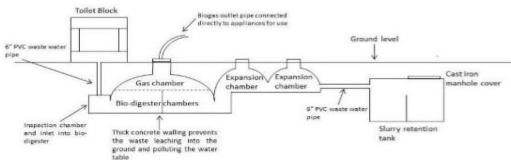
Figure 2: Bio-latrine installation constructed by Practical Action in Kitale, Kenya. Illustration: Practical Action.
