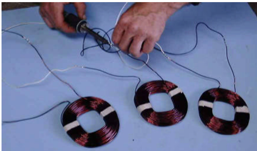
Some coils for the stator
