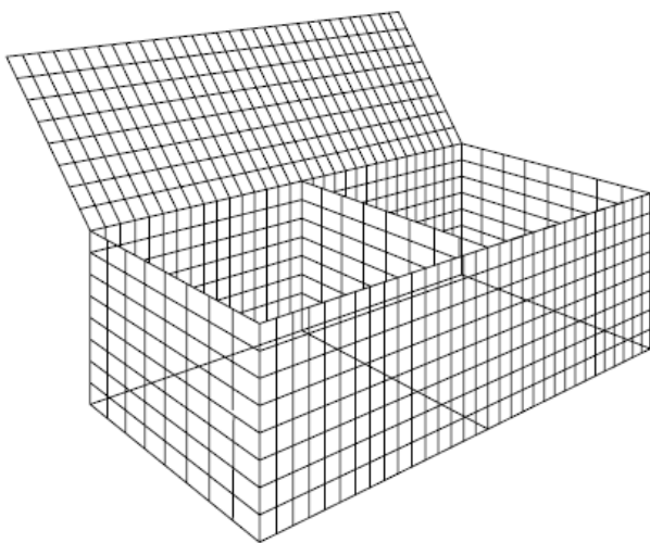
Figure 6: A basic gabion before loading with stones Illustration: Practical Action / Neil Noble.
