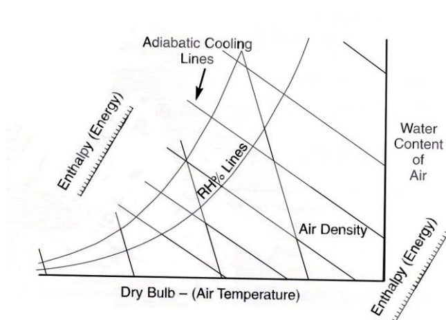
Figure 1: A simple psychrometric chart
