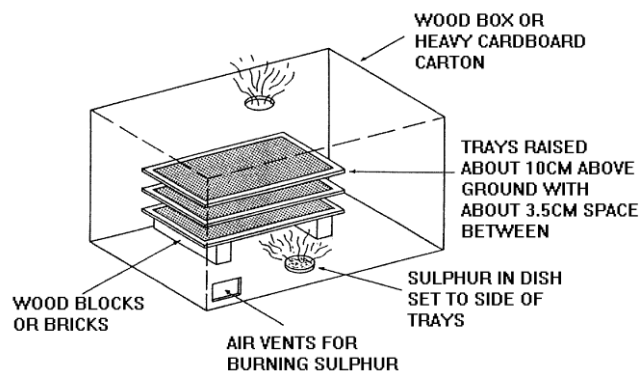
Figure 5: Sulphuring cabinet
